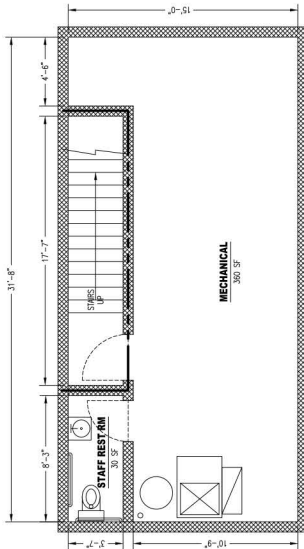
BASEMENT FLOOR PLAN SCALE: 3/4"
